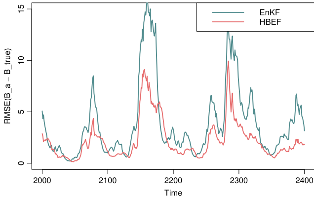
Fig. 5. RMSEs in B_k^a produced by the EnKF and the HBEF.
