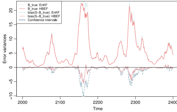
Fig. 3. The two lower curves: biases in the forecast ensemble variances (with the 95% confidence intervals) for the EnKF and the HBEF. The two upper curves: the respective true error variances B_k .
