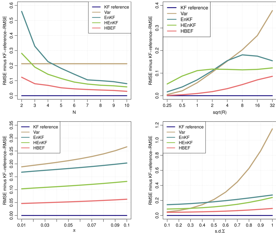
Fig. 4. The filters' analysis RMSEs of the state (with the reference-KF analysis RMSE subtracted) as functions of the ensemble size N (top, left), the observation error standard deviation \sqrt{R} (top, right), the degree of the system's intermittent instability \pi (bottom, left), the variability in the model error standard deviation s.d. \Sigma (bottom, right).
