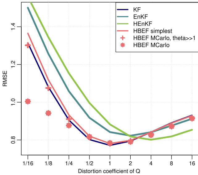
Fig. 6. Analysis RMSEs of the state for the filters which used the wrong Q . The latter was specified to be the true Q multiplied by the distortion coefficient q_{\text{distort}} .
