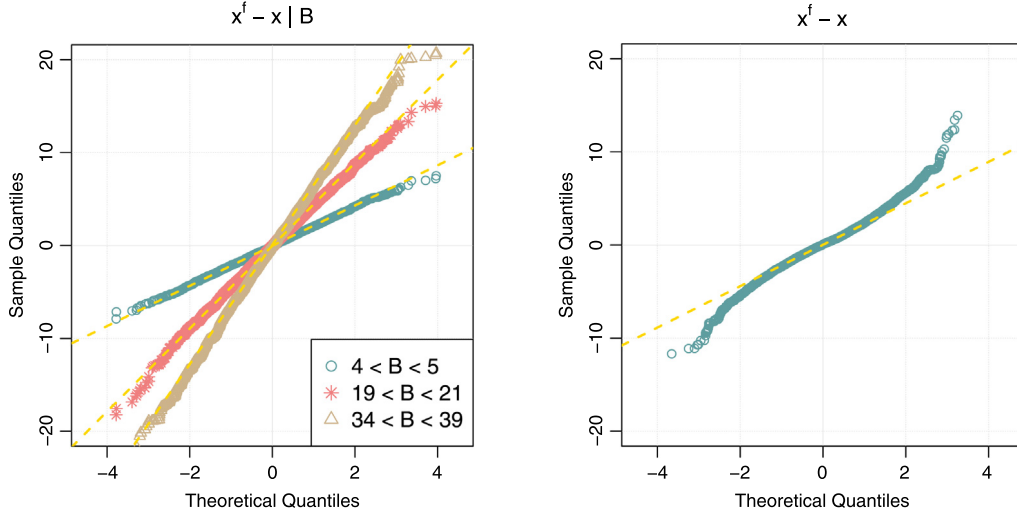
Fig. 2. The Gaussian q - q plots for the conditional pdf p(x_k^f - x_k | B_k) (left) and the unconditional pdf p(x_k^f - x_k) (right). In the left panel, the three curves correspond to the three intervals of B_k indicated in the legend.
