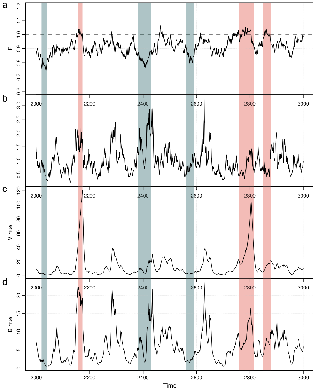
Fig. 1. Typical time series of: (a) The forecast operator F_k , (b) The model error standard deviation \sigma_k , (c) The variance of the truth V_k , and (d) The true background error variance B_k for the HBEF. The light gray (pink in the web version of the article) vertical stripes indicate events when F_k > 1 . The dark gray (blue in the web version of the article) vertical stripes indicate events when |F_k| was relatively low.
